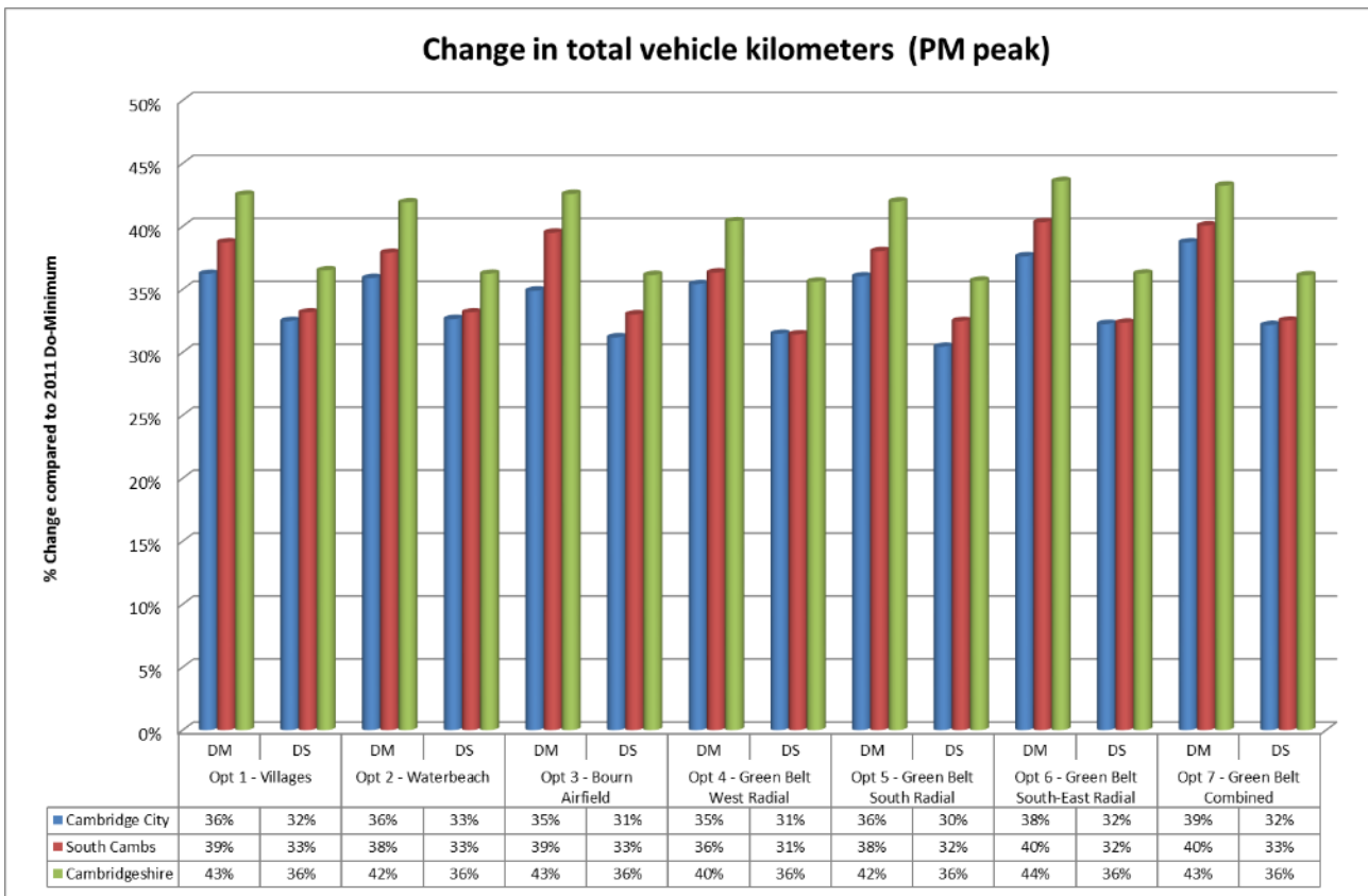
Figure 5-6 Change in total vehicle kilometers (PM peak)
