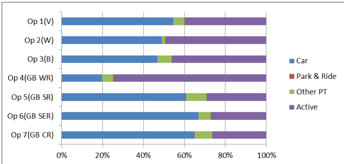
Figure 5-13 Mode Share of AM trips from major development areas to All Destinations (DS)
